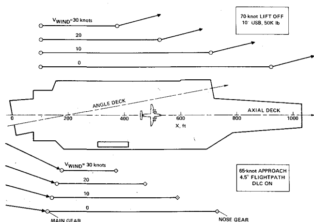
Fig. 12 Predicted carrier-deck requirements.
