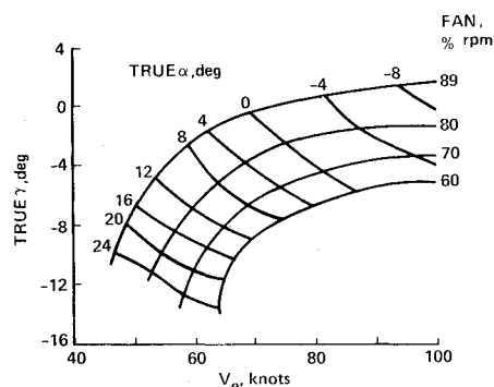
Fig. 7 Flight-path and angle-of-attack characteristics: all engines operating, double-slotted flaps deflected 59 deg, USB = 50 deg.
