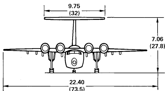
DIMENSIONS IN m (ft)
