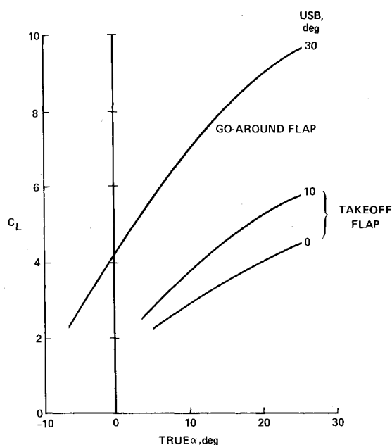
Fig. 3 Corrected lift coefficients: all engines operating at 89% rpm, double-slotted flaps deflected 59 deg.
