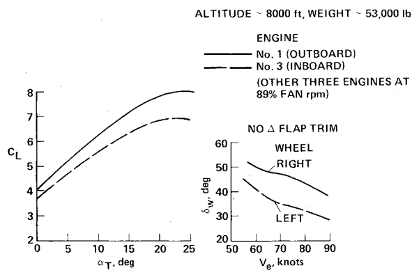
Fig. 6 Engine-out characteristics: double-slotted flaps deflected 59 deg, USB = 55 deg.
