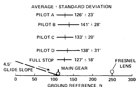
Fig. 10 Touchdown dispersion.
