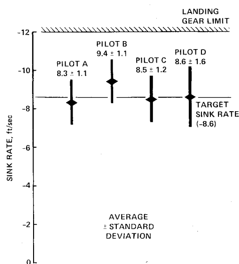
Fig. 11 Touchdown sink rates.
