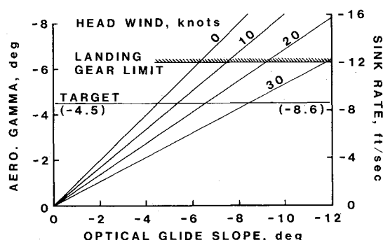
Fig. 9 65-knot approach planning chart.
